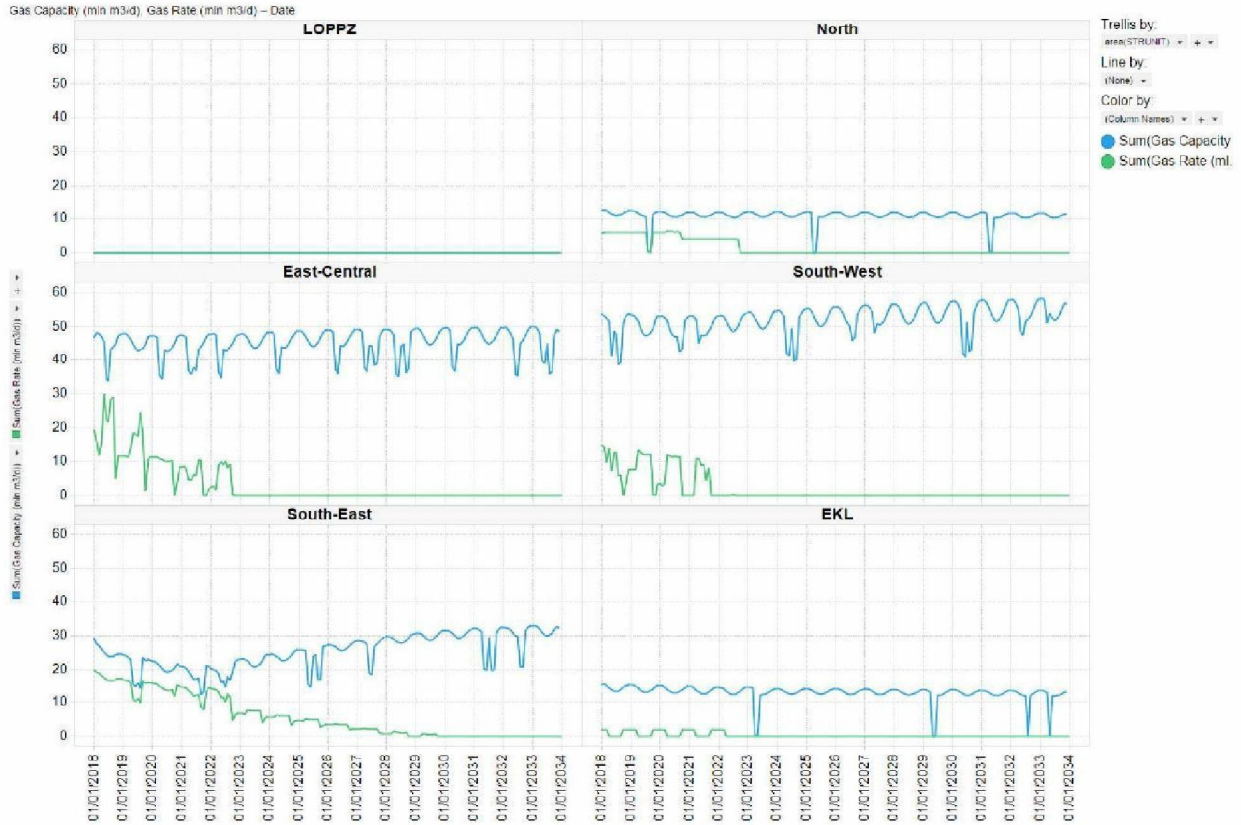
Figure 3-15: Forecasted production (green lines) and capacity (blue lines) per region for warm temperature
