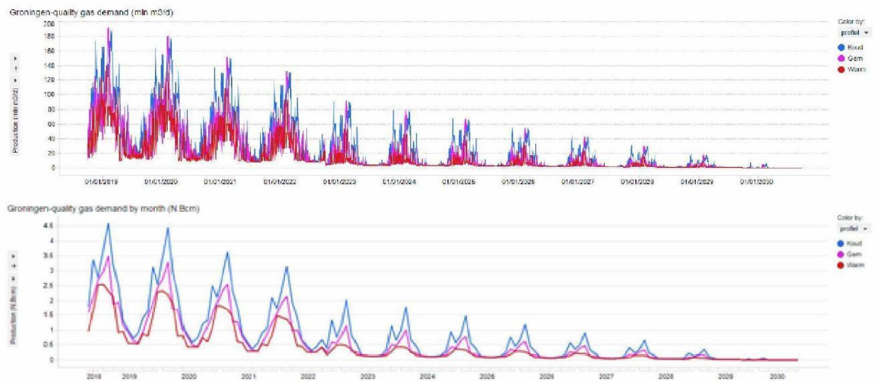
Figure 2-1 Groningen quality market demand in excess to the other L-gas supply sources for a sequence of cold, average and warm temperatures years. Top graph represents daily volume and bottom graph reflects monthly demand volume.
