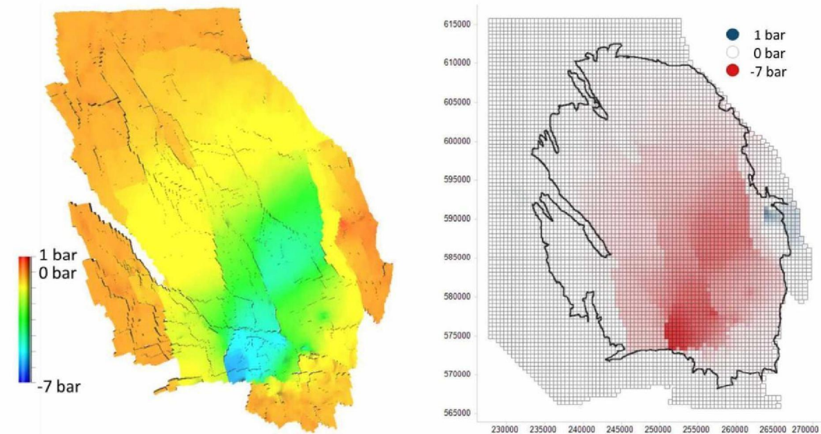
Figure 3-14: Incremental reservoir pressure decline for Warm scenario as compared to the Average temperature scenario, between 1/1/2018 and 1/1/2023.
