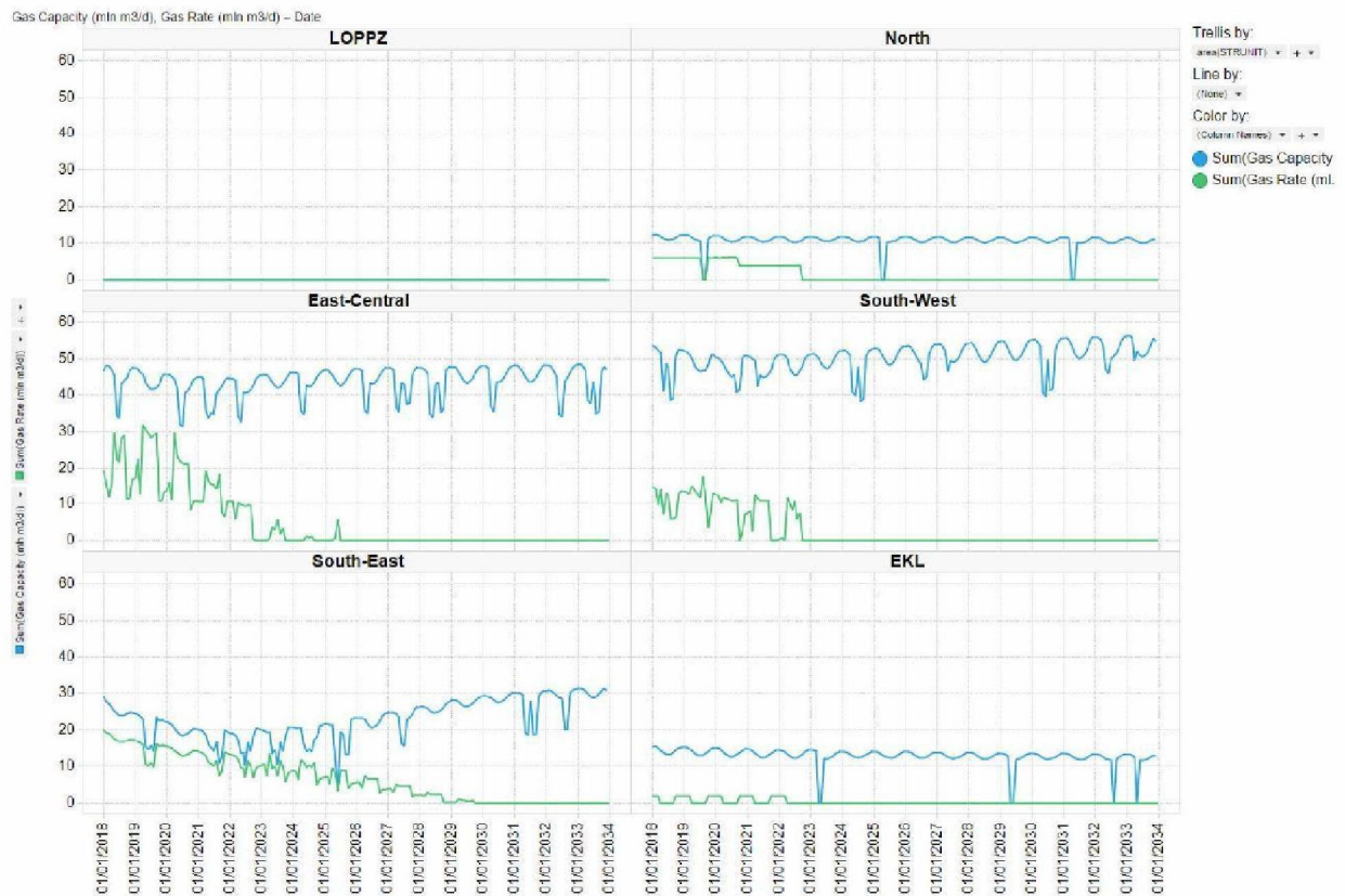
Figure 3-5: Forecasted production (green lines) and capacity (blue lines) per region for average temperature
