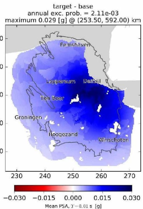
Figure 4-8b Cold-temperature scenario -- annual hazard plots (left) and difference w.r.t. corresponding average-temperature scenario hazard (right)
