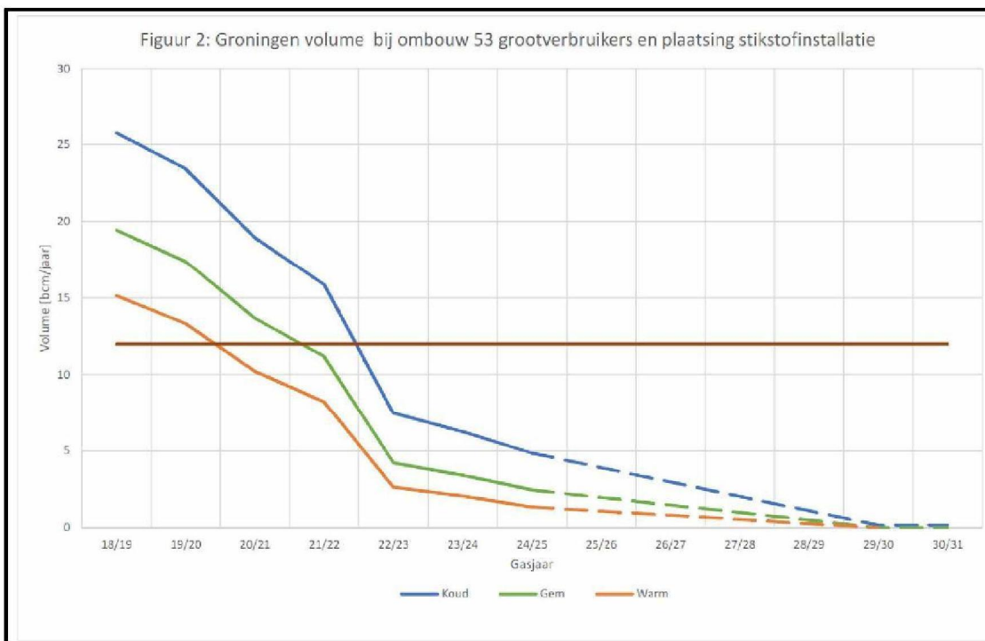
Figure 1.2 Production scenario "Basispad Kabinet" for a sequence of cold temperature years (in blue), average temperature years (in green) and of warm temperature years (in orange) from refence 7.
