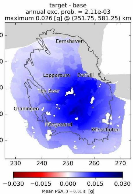
Figure 4-8a Cold-temperature scenario -- annual hazard plots (left) and difference w.r.t. corresponding average-temperature scenario hazard (right)
