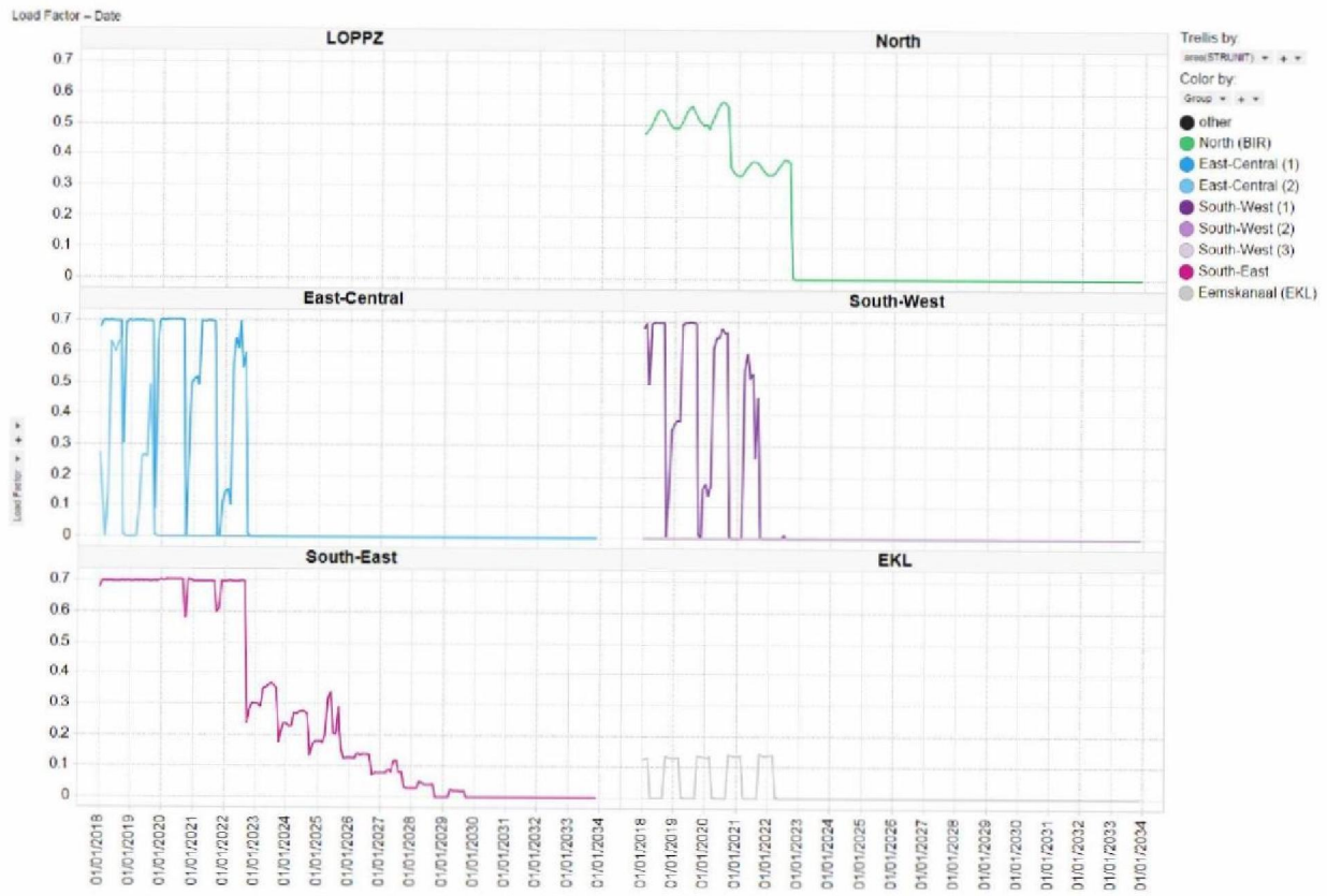
Figure 3-16: Load Factor per region and start-up group
