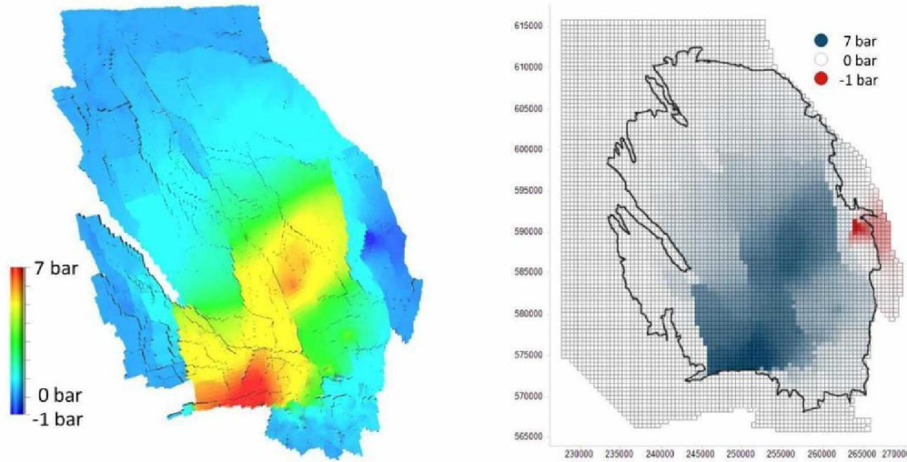
Figure 3-9: Incremental reservoir pressure decline for Cold scenario as compared to the Average temperature scenario, between 1/1/2018 and 1/1/2023.
