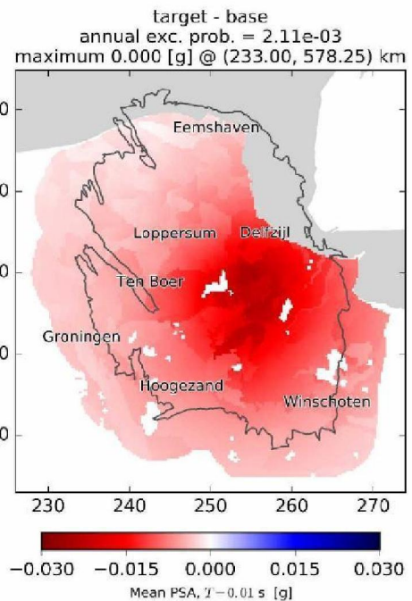
Figure 4-9a Warm-temperature scenario -- annual hazard plots (left) and difference w.r.t. corresponding average-temperature scenario hazard (right)
