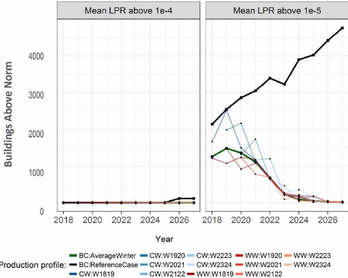
Figure 5.4 Graphs show the Local Personal Risk associated with the production scenario "Basispad Kabinet" for average (green), cold weather and warm weather years, and the Reference Scenario (24 Bcm/year) (black), and for the period 2018 to 2027. Each cold (blue) and warm (red) year is followed by average temperature years. Right graph: number of buildings exceeding the norm mean LPR larger than 10^{-5} /year Left graph: number of buildings exceeding the norm mean LPR larger than 10^{-4} /year
