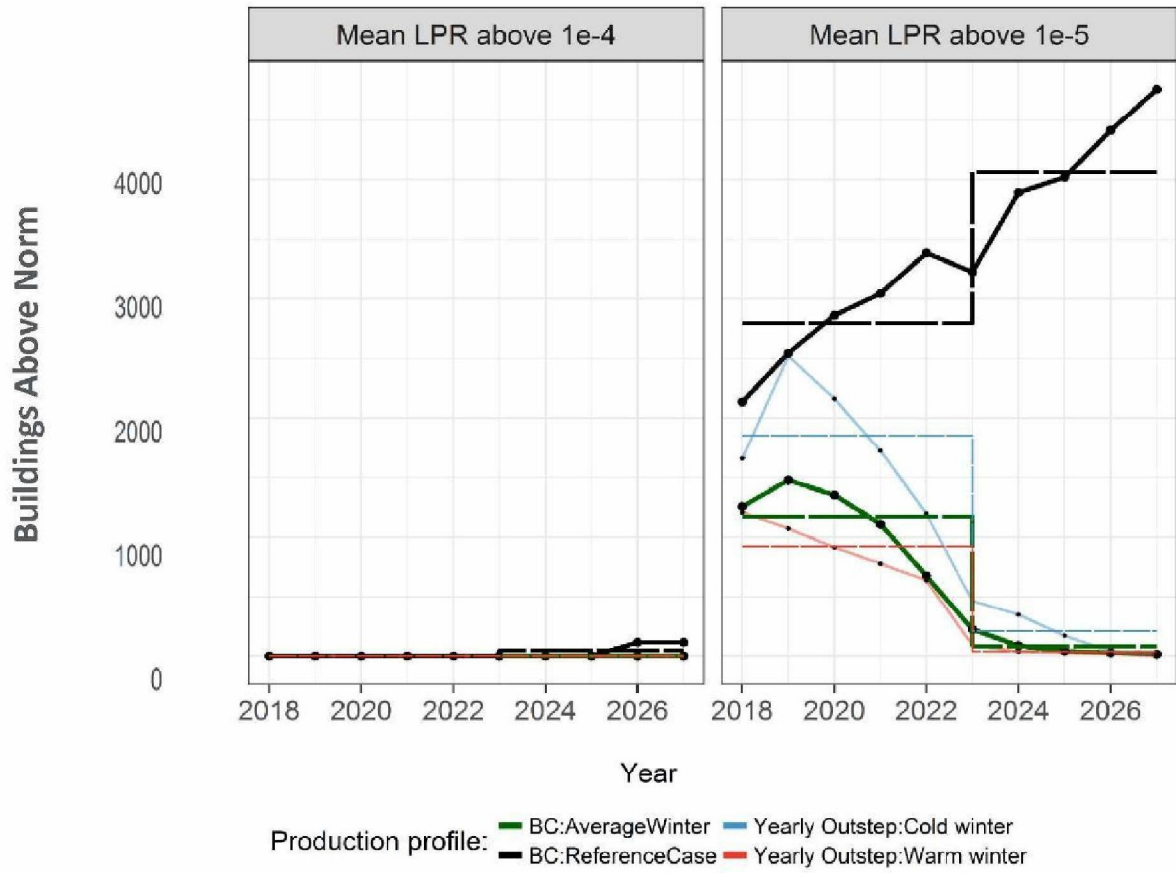
Figure 5.5 Graphs show the Local Personal Risk associated with the production scenario "Basispad Kabinet" for average (green), cold weather and warm weather years, and the Reference Scenario (24 Bcm/year) (black), and for the period 2018 to 2027. The cold and warm weather years have been gathered as the blue and red line respectively. Right graph: number of buildings exceeding the norm mean LPR larger than 10^{-5} /year Left graph: number of buildings exceeding the norm mean LPR larger than 10^{-4} /year
