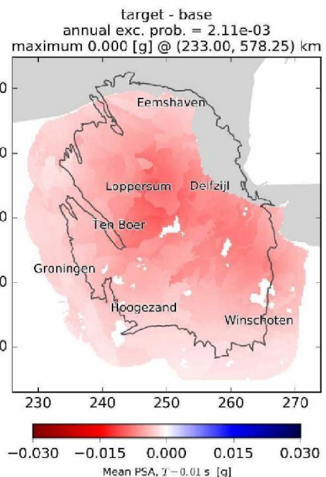
Figure 4-9b Warm-temperature scenario -- annual hazard plots (left) and difference w.r.t. corresponding average-temperature scenario hazard (right)
