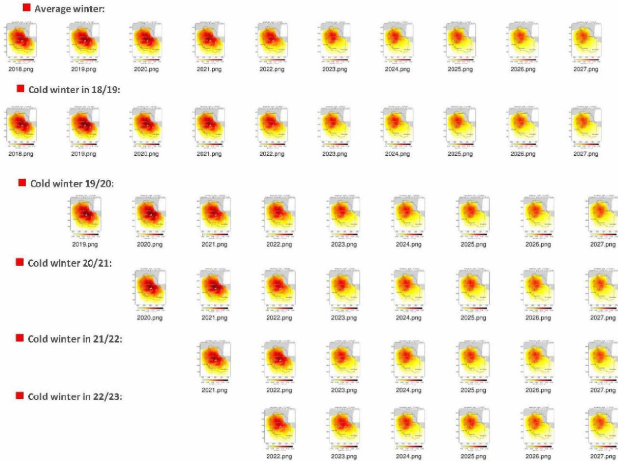
Figure 4-7 Hazard maps for the average winter weather scenario (top) followed by the different cold weather cases making up de cold weather scenario. Gas-year 2018/2019 as a cold year followed by average temperature years (second line). Gas-year 2019/2020 as a cold year followed by average temperature years (third line). Following lines start with cold year followed by average temperature years.
