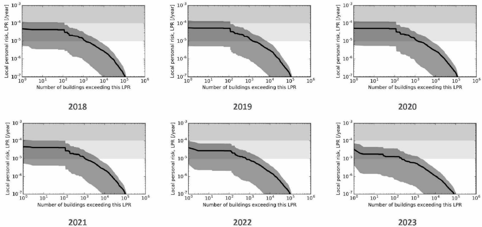
Figure 5.1a Local Personal Risk graphs for the years 2018 to 2023. These show the number of houses that are exposed to a LPR. The black lines denote the mean and the dark grey areas the uncertainty bands. The two horizontal bands in light grey denote the LPR levels of the Meijdam-Norm.
