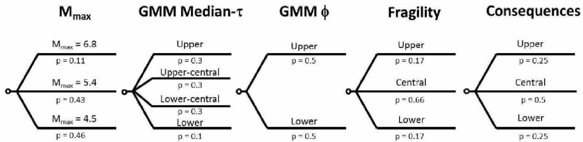
Figure C.1 Summary of the logic-tree used to characterise epistemic uncertainties within the Probabilistic Seismic Hazard and Risk Analysis. The complete logic tree contains 216 branches which comprises the full factorial combination of these 5 factors and their associated 2–4 levels. Each logic tree branch was analysed by an independent Monte Carlo simulation of the unique combination of sub-models. Mean hazard and risk metrics are derived as the probability-weighted combination of all Monte Carlo results across the complete logic tree.
