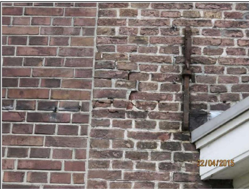
Schade 19, Scheuren in metselwerk (57784 22-4 (194))
