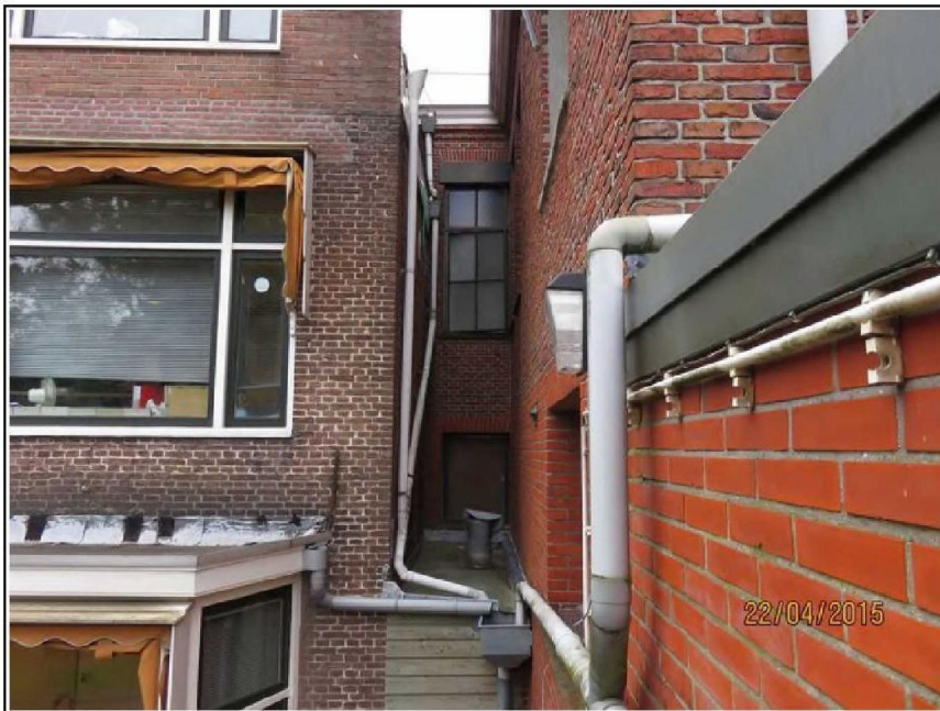
Schade 19, Scheuren in metselwerk (57784 22-4 (189))
