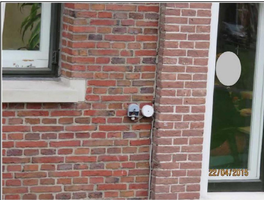
Schade 2, Verticale scheur (57784 22-4 (14))
