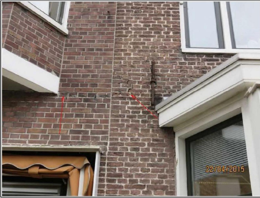
Schade 19, Scheuren in metselwerk (57784 22-4 (193))
