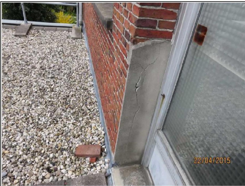
Schade 17, Verticale scheurn (57784 22-4 (186))
