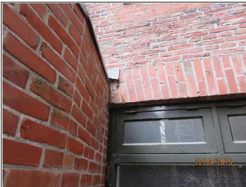
Schade 8, Scheurvorming in metselwerk (57784 22-4 (109))
