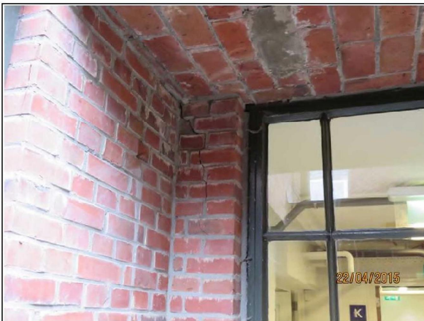
Schade 8, Scheurvorming in metselwerk (57784 22-4 (106))
