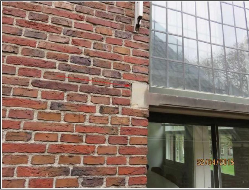
Schade 3, Verticale en horizontale scheuren (57784 22-4 (65))
