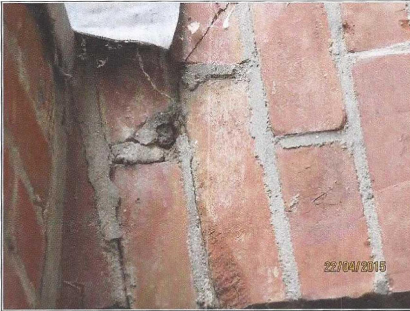
Schade 8, Scheurvorming in metselwerk (57784 22-4 (110))
