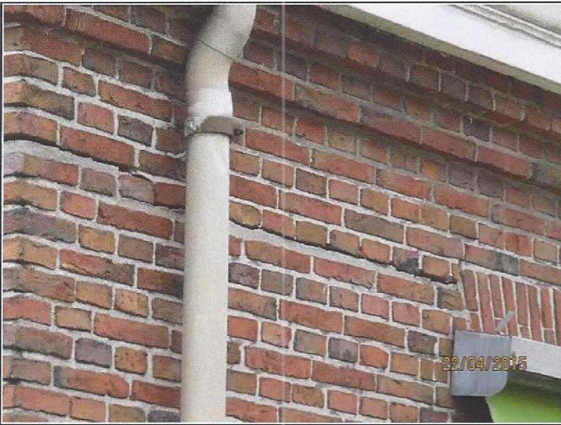
Schade 16, Horizontale scheuren. (57784 22-4 (174))
