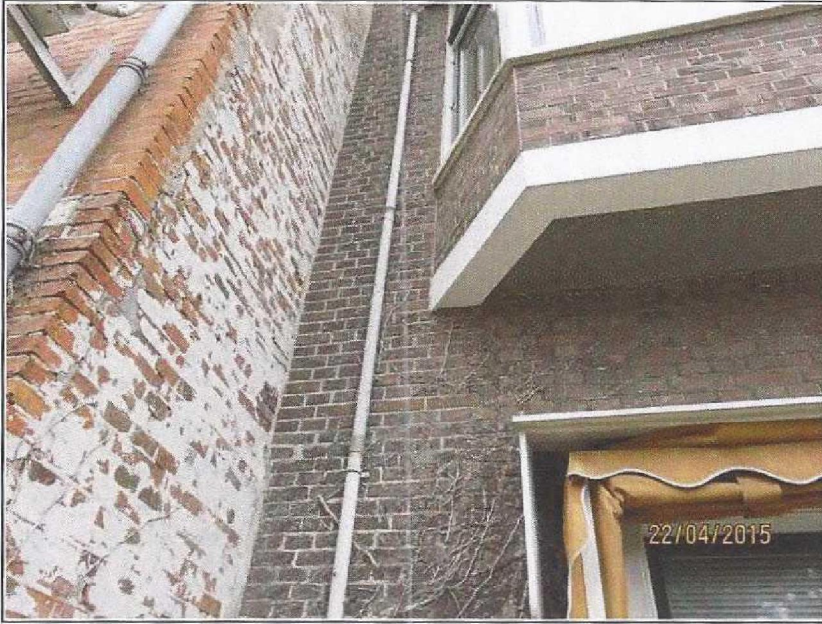
Schade 19, Scheuren in metselwerk (57784 22-4 (197))
