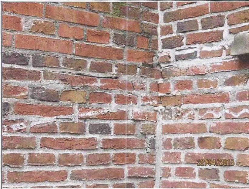
Schade 9, Scheurvorming in metselwerk (57784 22-4 (116))
