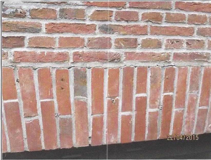
Schade 9, Scheurvorming in metselwerk (57784 22-4 (114))
